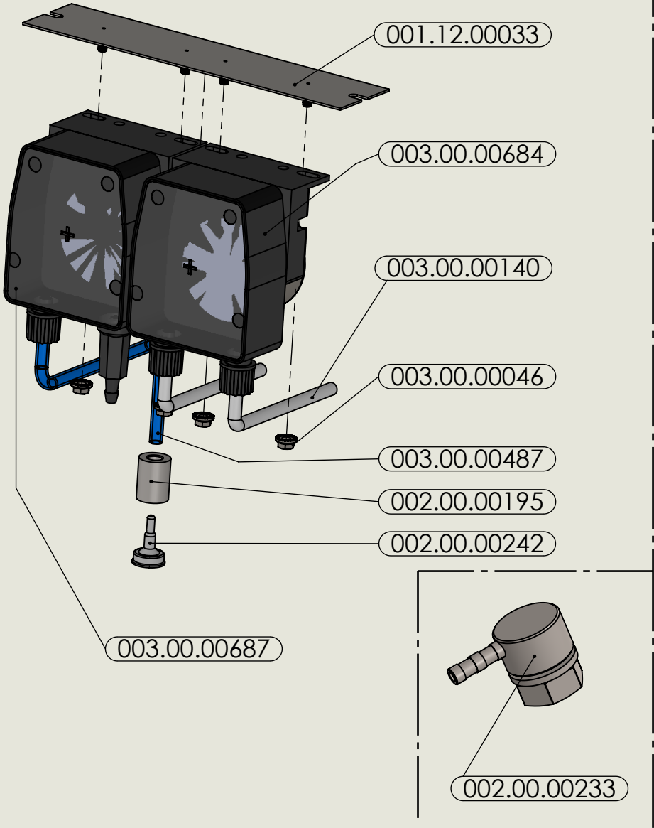
003.00.00734 PUMP KIT
