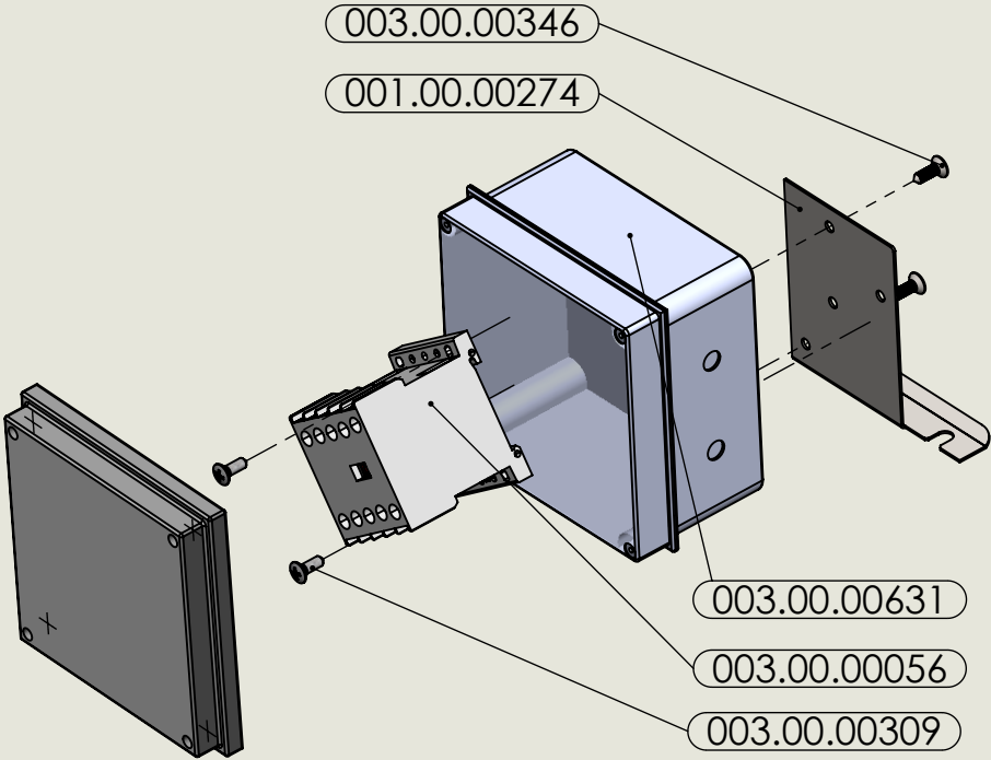
006.00.00000 COMPONENT SET
