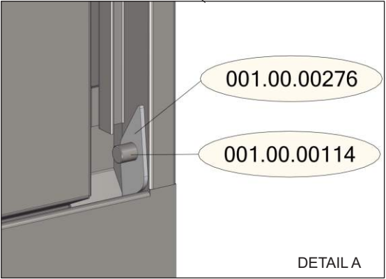
DOOR SUPPORT
