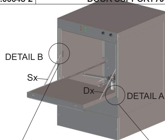
DOOR SUPPORT
